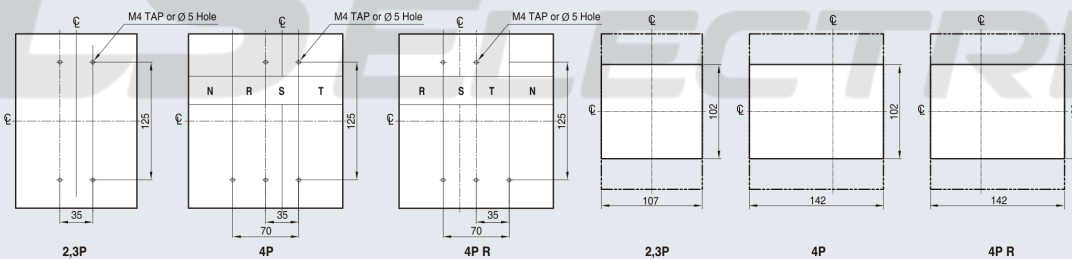
Front panel cutting
