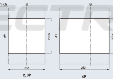
Front panel cutting
