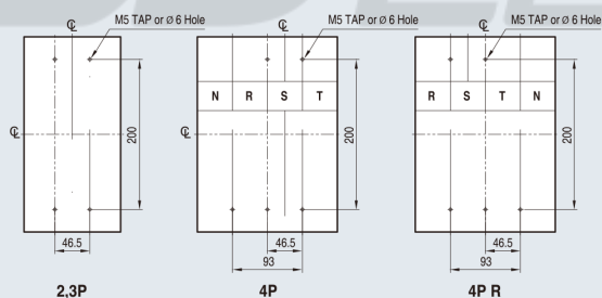
Panel drilling
